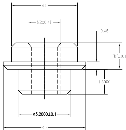
STAND OFF
