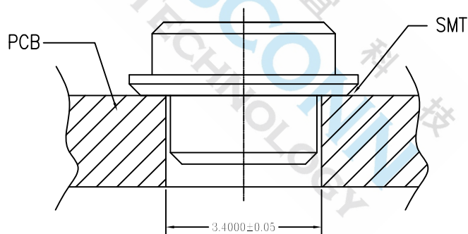
PCB Layout Recommended
